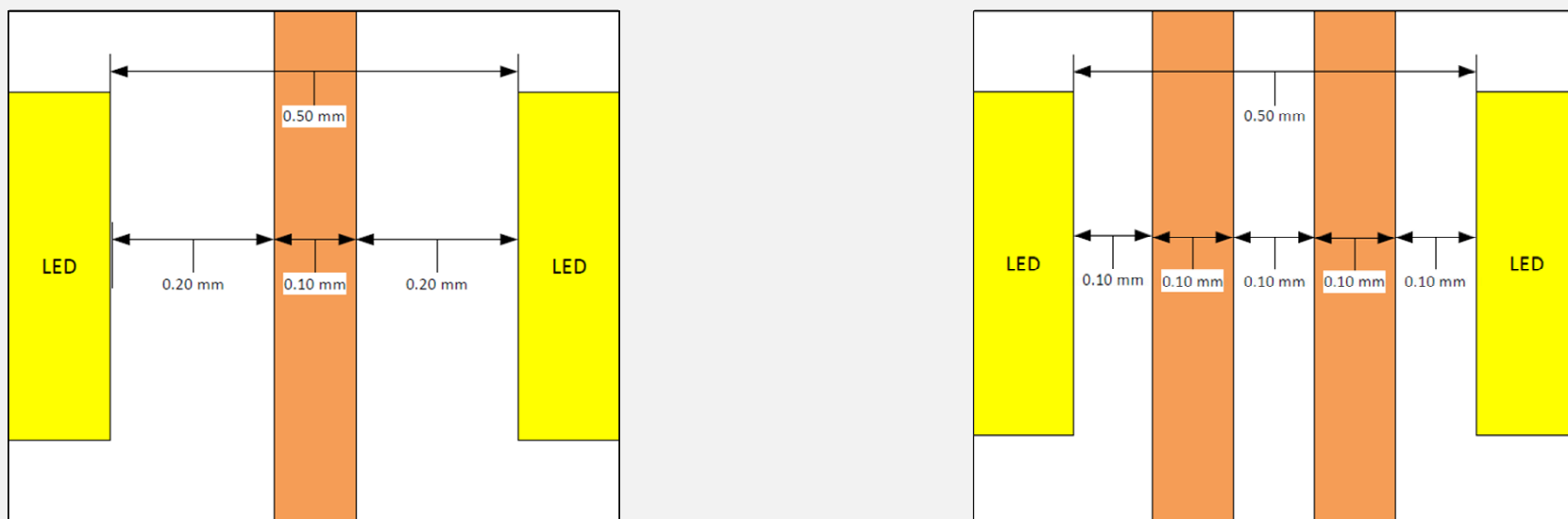
Fig. 5 Minimum track and gap between LED positions.
